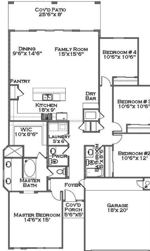
FLOOR PLAN
