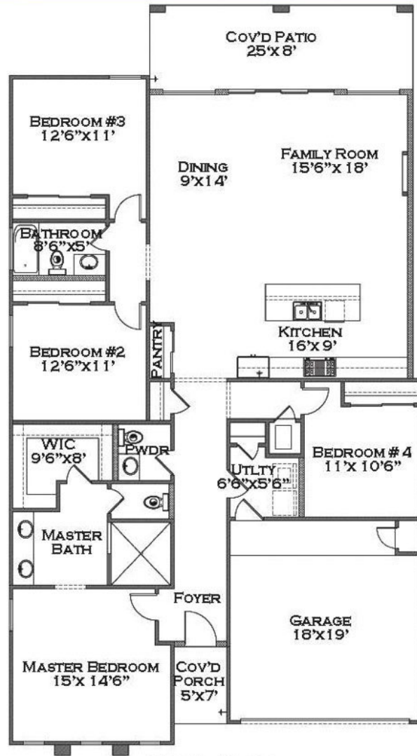
FLOOR PLAN
